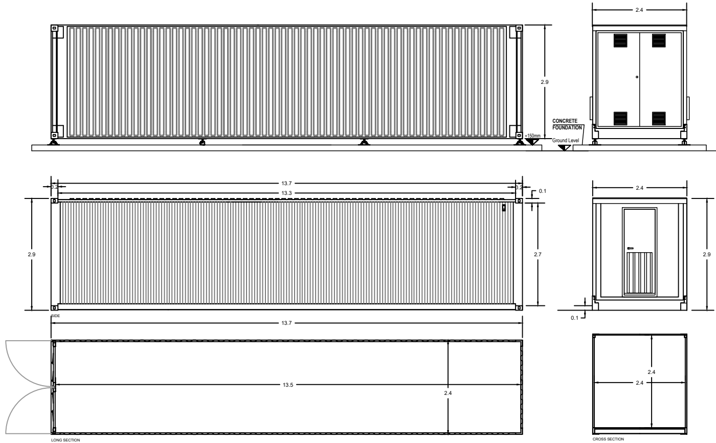
Battery Storage Elevations (TYPICAL) Light Gray/ Dark Green metal
